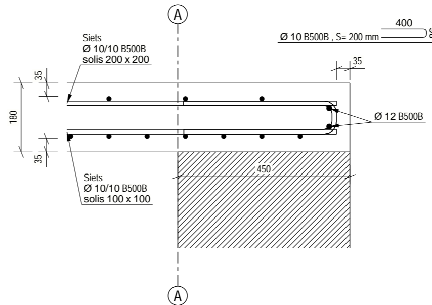
DETAIL A 1:10
